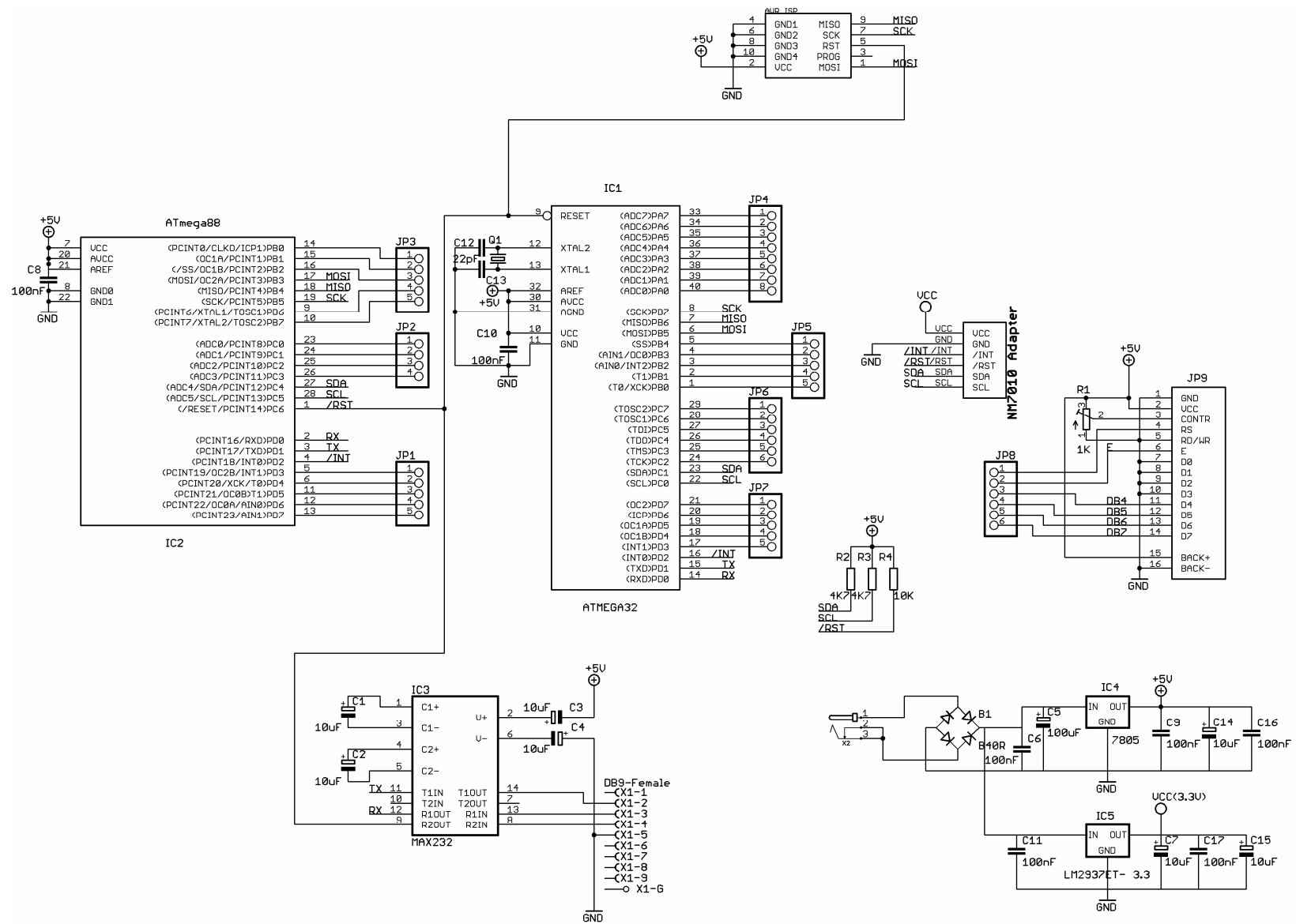
Mother Board
