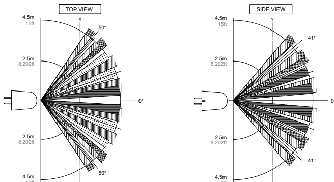
X-Y cross section
