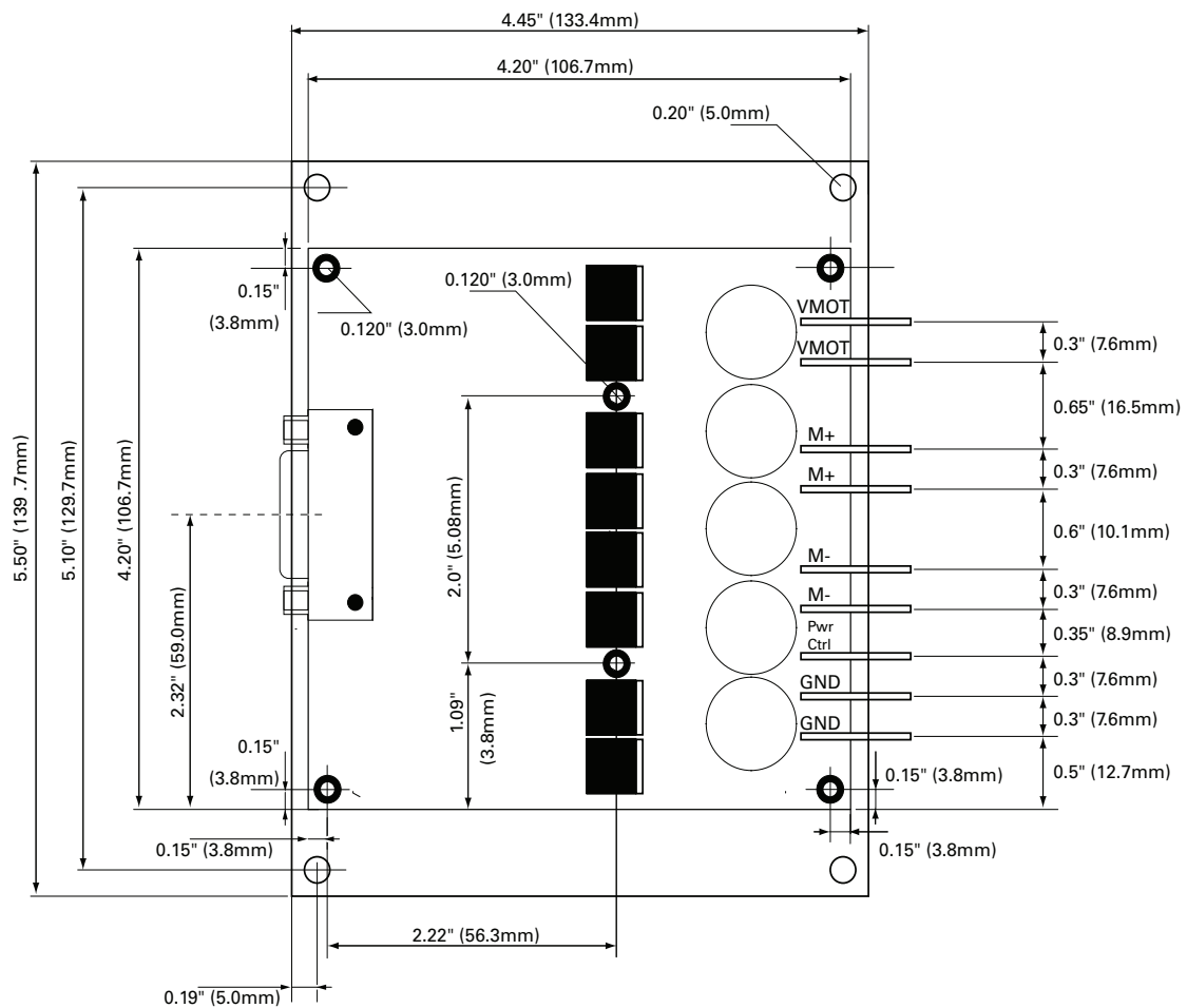
FIGURE 16. MDC14xx top view and dimensions
