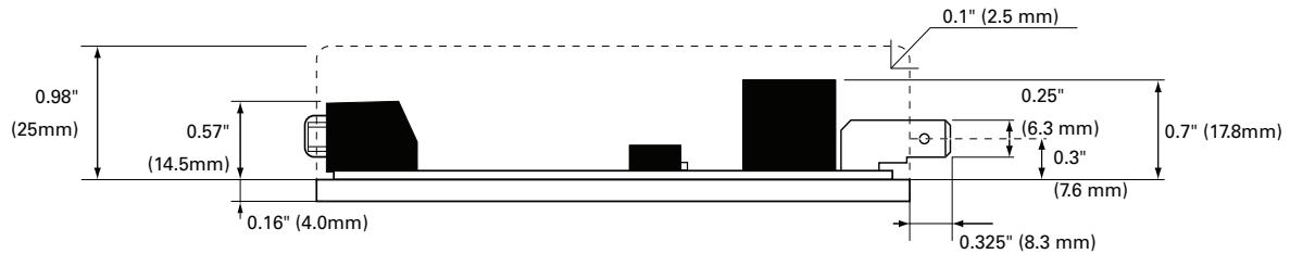
FIGURE 15. MDC14xx front view and dimensions
