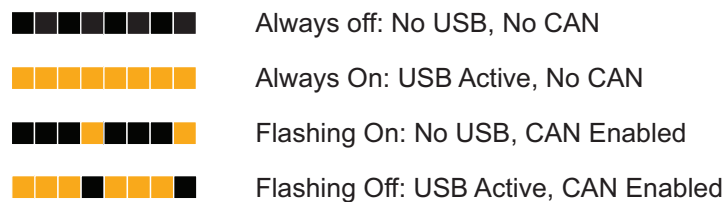
FIGURE 9 Communication LED
