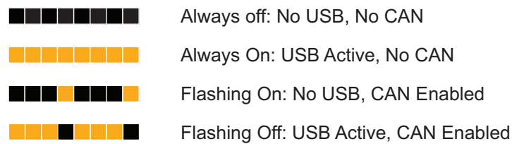
FIGURE 9. Communication LED
