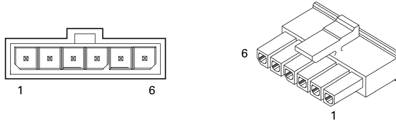
FIGURE 5. Encoder connector
