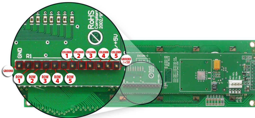
Figure 18: Keypad Interface Connector
