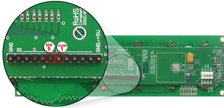
Figure 17: Manual Override Jumper
