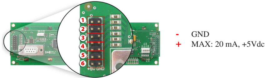
Figure 15: General Purpose Output
