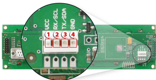
Figure 13: Power Connector and Pin out
