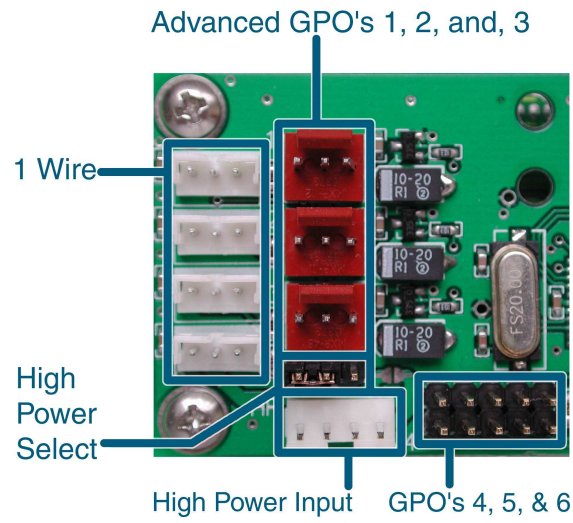
Figure 7: Connections
