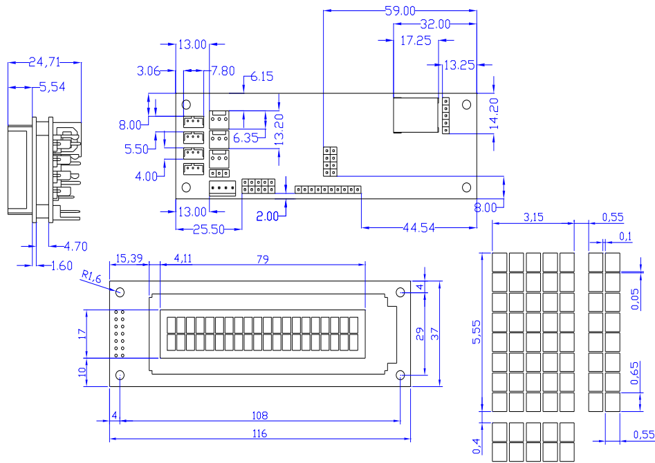
Figure 15: Physical Layout
