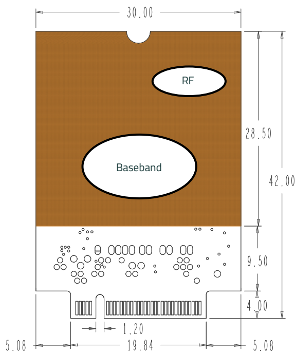
Figure 6-2: Copper Pad Location on Bottom Side of Module
