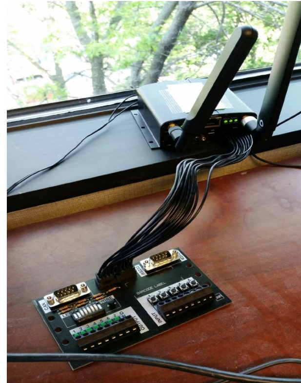
CloudGate with telematics card installed + breakout card and cable
