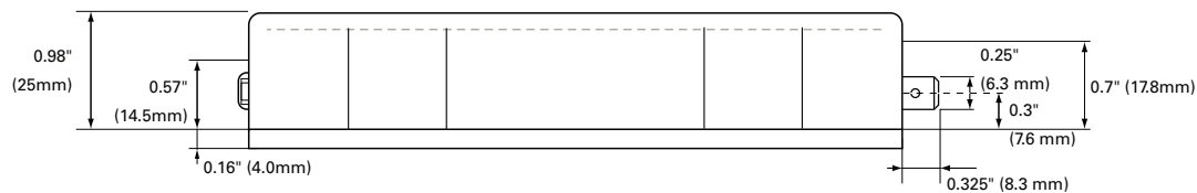
FIGURE 13. FIM2360 side view and dimensions
