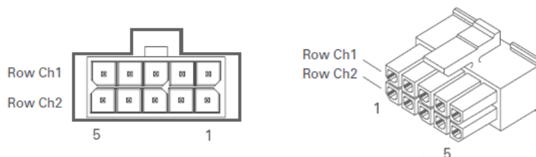
FIGURE 6. Encoder connector
