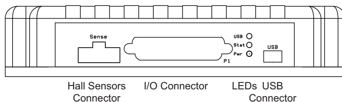
FIGURE 1. FBL2360 front view
