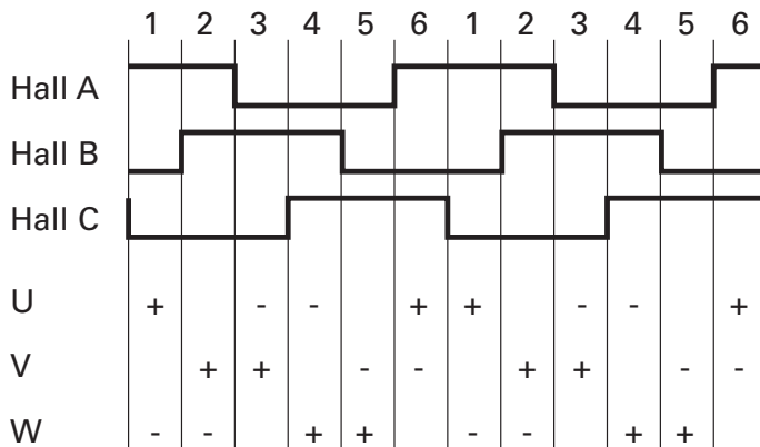
FIGURE 7. Hall Sensors sequence
