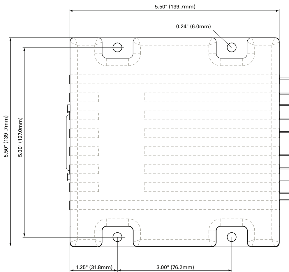
FIGURE 14. FBL2360 top view and dimensions
