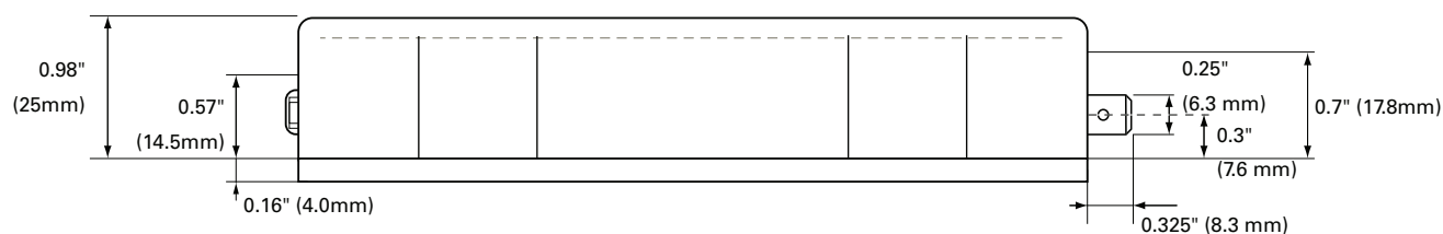
FIGURE 13. FBL2360 side view and dimensions
