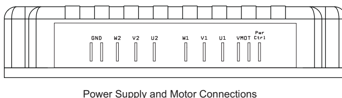
FIGURE 2. FBL2360 rear view
