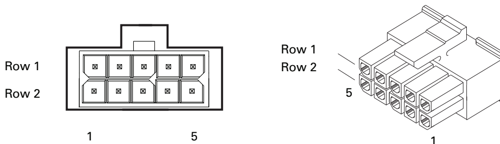
FIGURE 8. Hall Sensor connector used for SPI encoders
