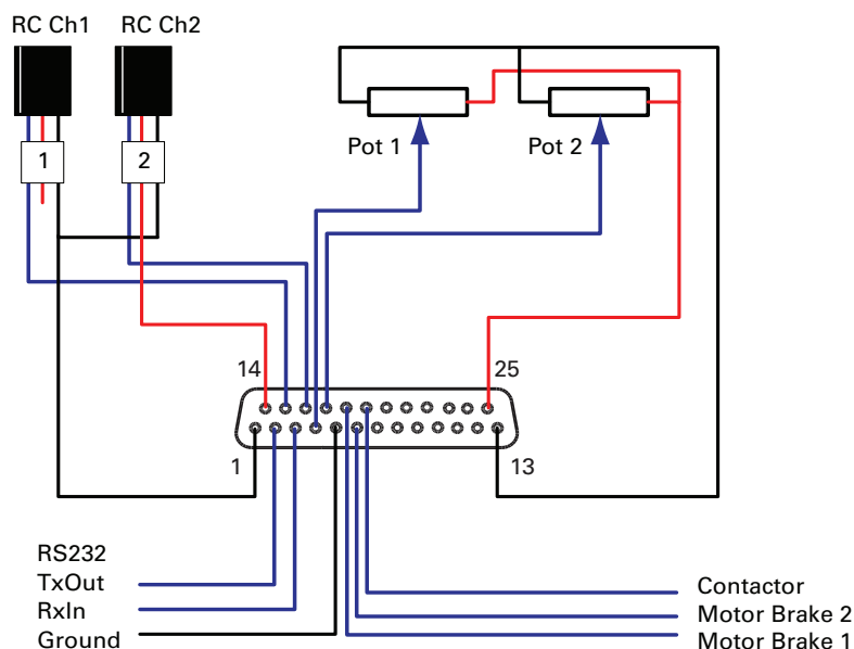
FIGURE 10. Factory default pins assignment
