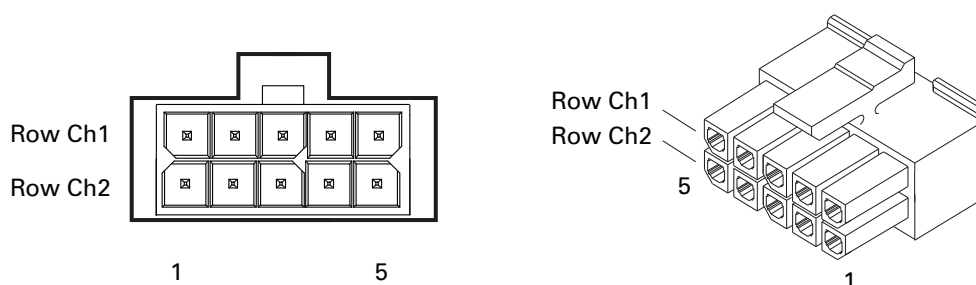
FIGURE 6. Hall Sensors connector
