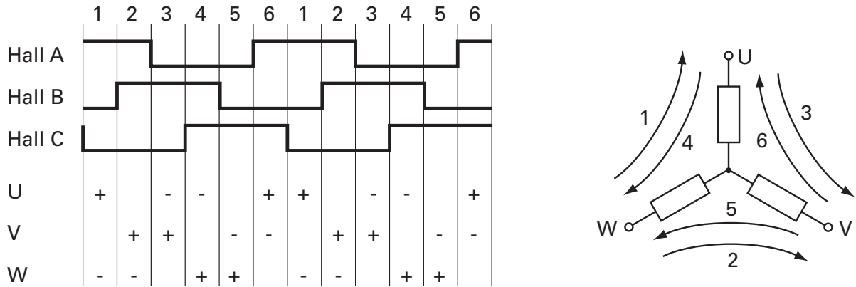
FIGURE 8. Hall Sensors sequence
