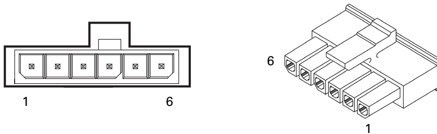
FIGURE 7. Hall Sensors connector
