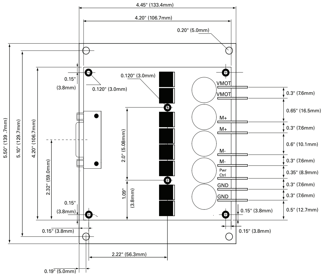
FIGURE 16. LDC14xx top view and dimensions
