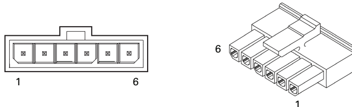
FIGURE 7. Hall Sensor connector used for SSI encoders
