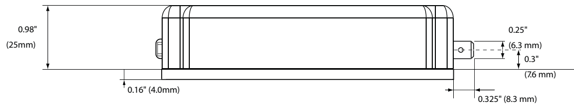
FIGURE 11. MBL1xxx side view and dimensions
