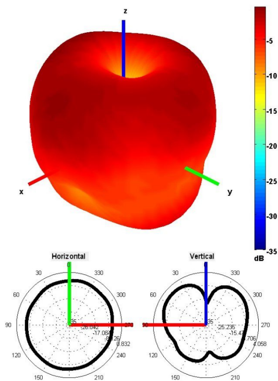
750 and 850 MHz Radiation pattern
