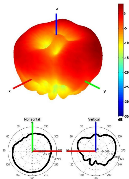
Cable 2: CELLULAR/LTE
