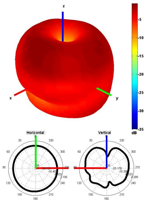
Cable 2: CELLULAR/LTE
