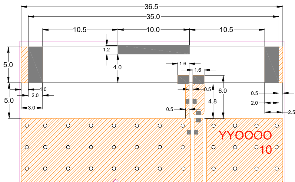
Layout dimensions for antenna integration (mm)
