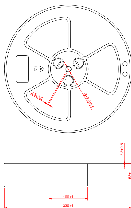
Tape and Reel Specifications
