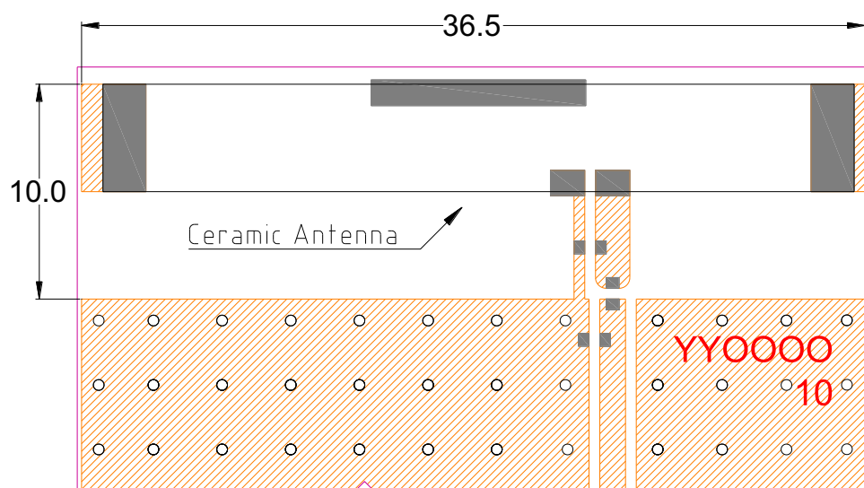
Minimum area required for antenna integration (44.8mm × 10mm)
