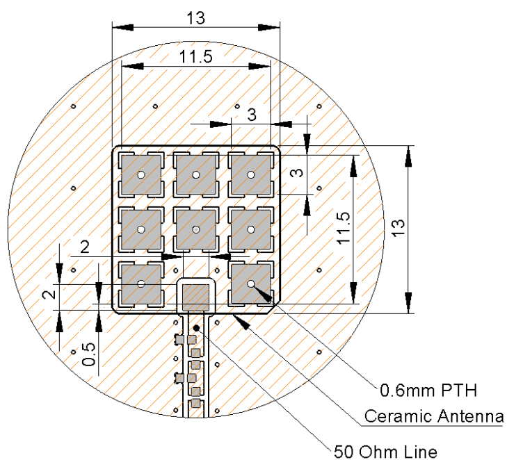
Layout dimensions for antenna integration (mm)
