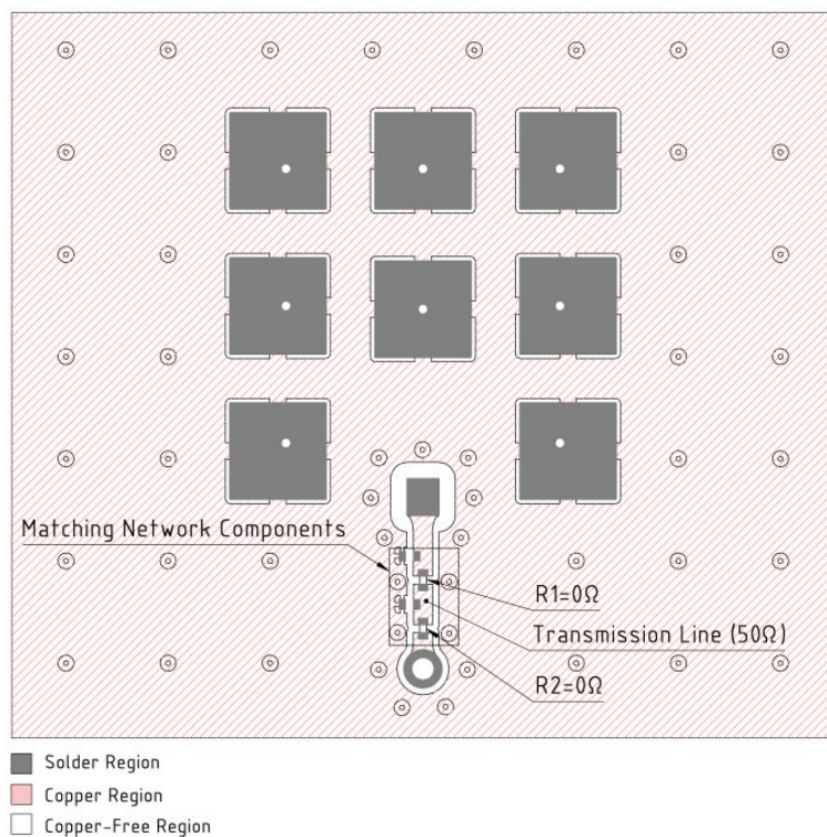
Matching Network Drawing
