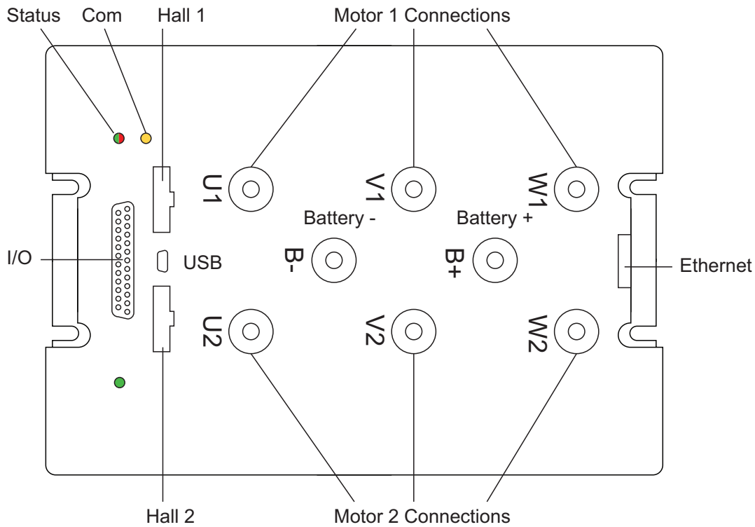
FIGURE 1. GBL26xx Rear View
