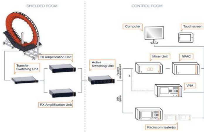
Measurement setup inside of radio chamber
