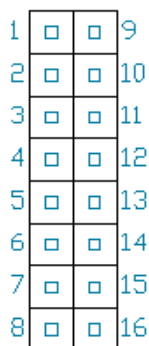
Figure 14: GPIO Header
