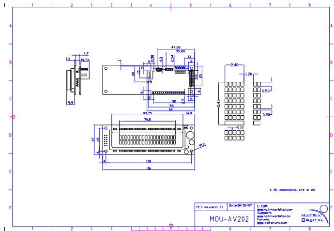
Figure 12: Physical Diagram
