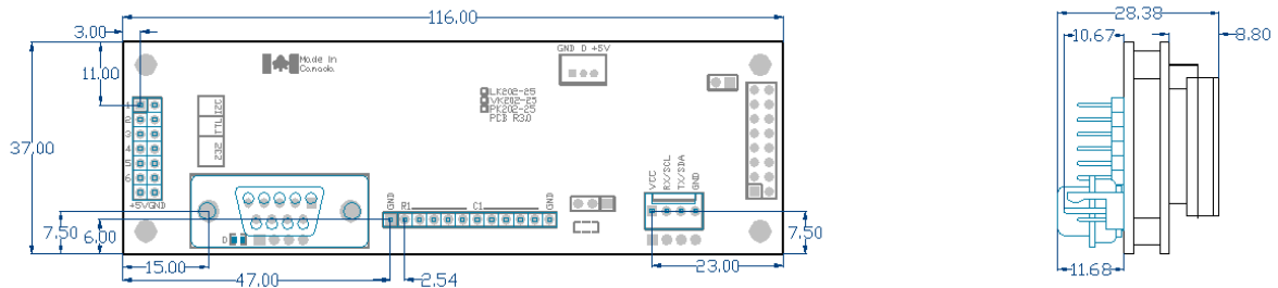
Figure 21: VK202-25 Dimensional Drawing
