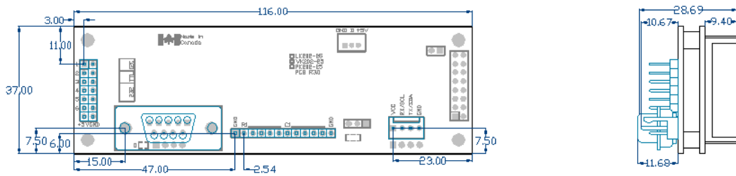
Figure 20: LK202-25 Dimensional Drawing
