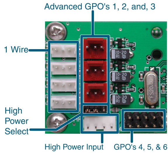
Figure 7: Connections
