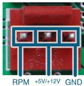
Figure 8: Fan Headers
