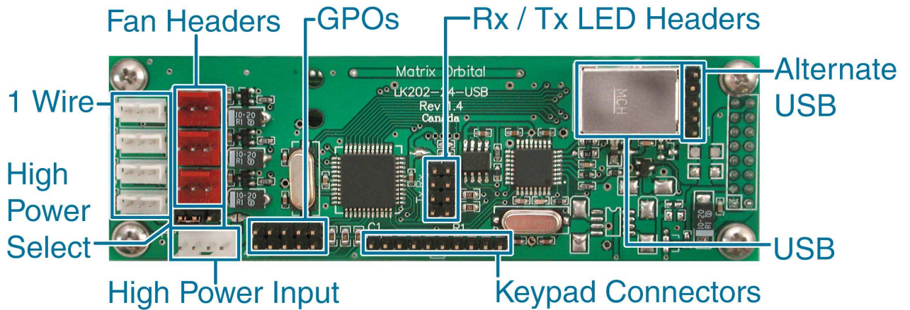
Figure 2: Electrical Connections
