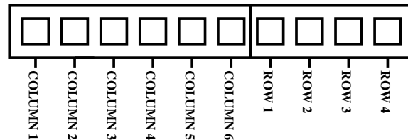
Figure 13: Keypad Connector
